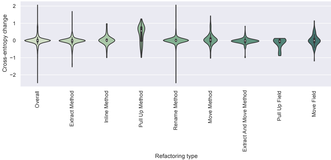
Fig. 1. Cross-entropy change after refactoring
